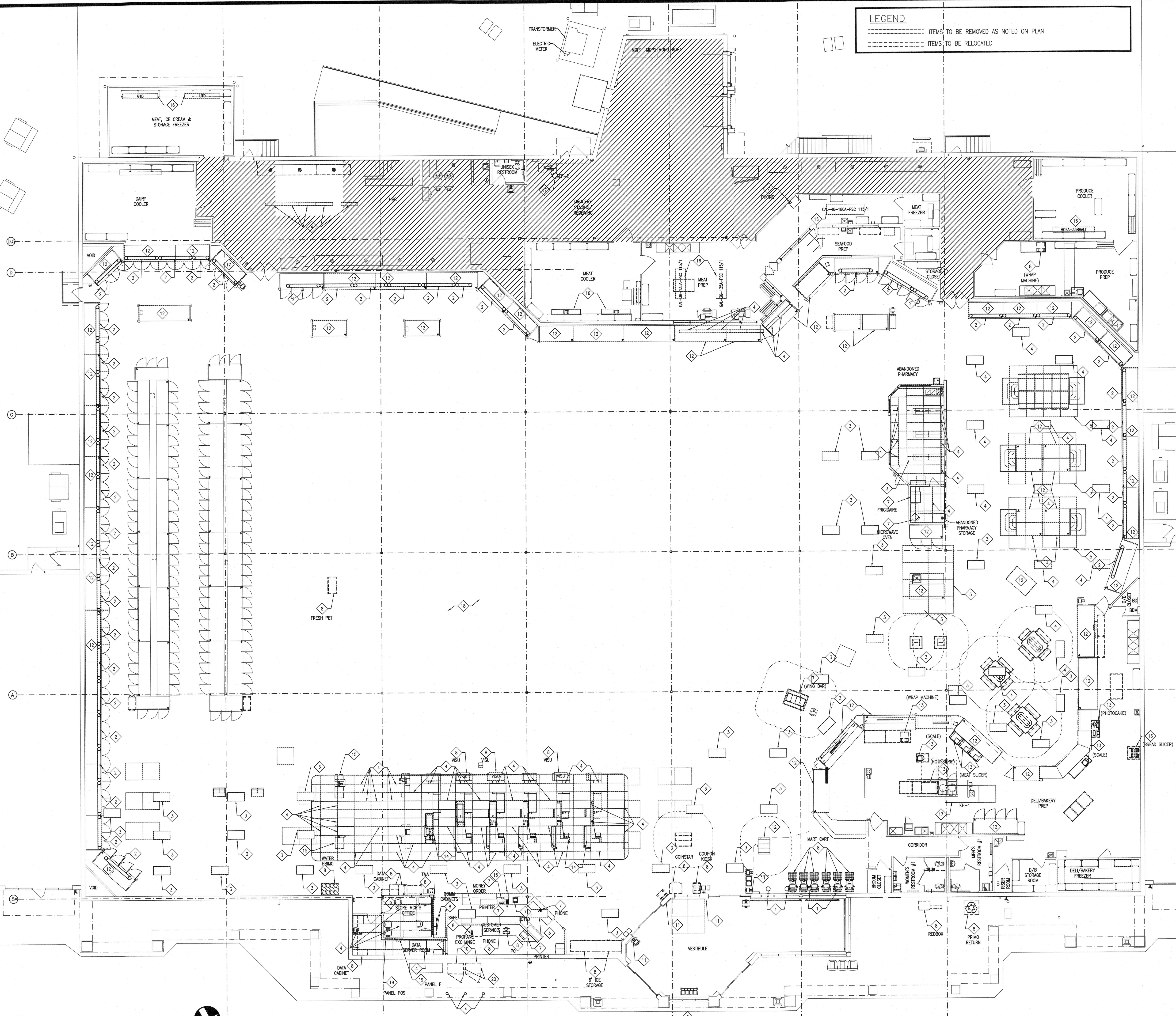
1 ELECTRICAL DEMOLITION PLAN E0.01 SCALE: 3/32" = 1'-0"
