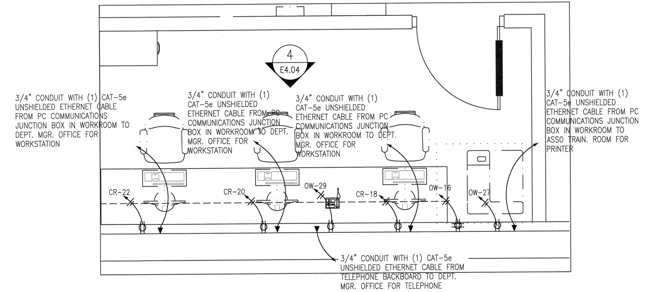
1 ENLARGED ELECTRICAL POWER PLAN - ASSO. TRAIN. ROOM E4.04 SCALE: 1/2" = 1'-0"
