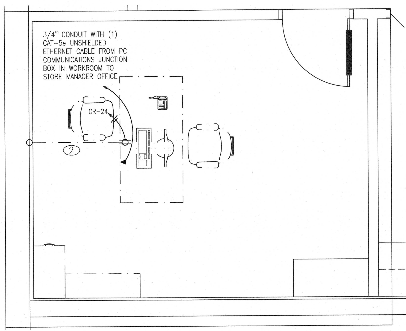
2 ENLARGED ELECTRICAL POWER PLAN - STORE MANAGER OFFICE E4.04 SCALE: 1/2" = 1'-0"
