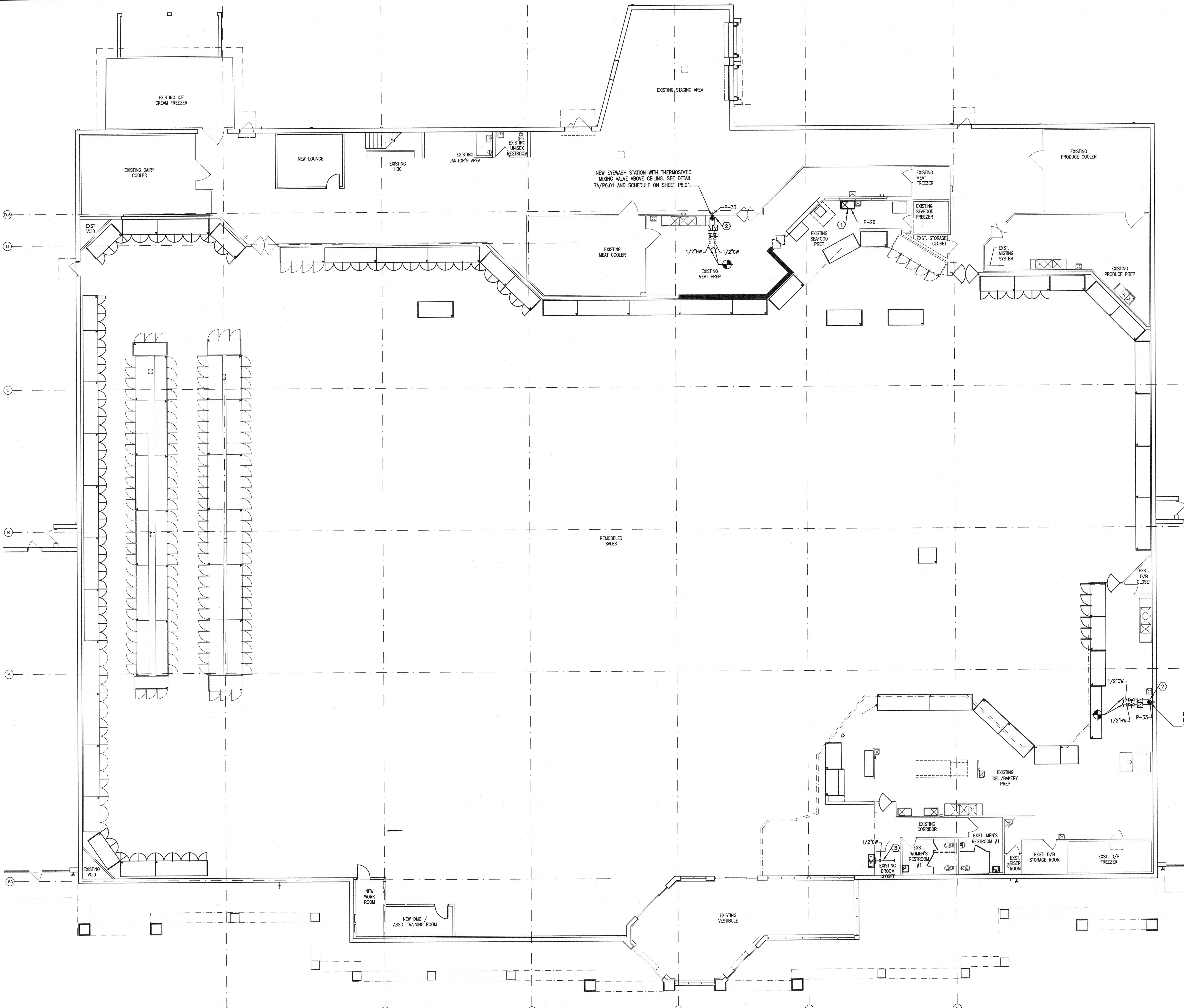
1 WATER PIPING PLAN P1.03 SCALE: 3/32" = 1'-0"
